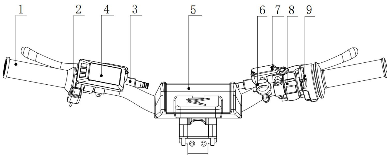
1-Grips 2-Horn 3-Left Lever(Rear Brake) 4-Dash 5-Chest Protector(Optional) 6-Magnetic Safety 7-Right Lever (Front Brake) 8-One-touch Ignition Switch 9-Throttle
